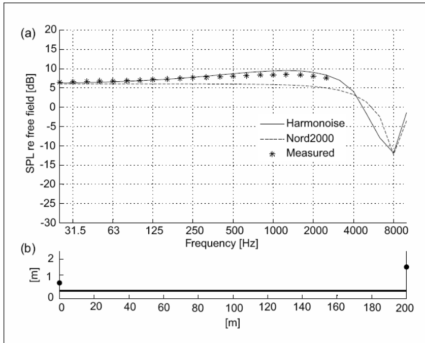
Figure 4. (a) Predicted results compared with reference data for test case 4: Sound propagation over 200 m of flat, acoustically hard ground with downwards refraction caused by a temperature gradient and no turbulence. Source height: 0.5 m; receiver height: 1.5 m; temperature gradient: 0.0846 K/m. (b) Terrain profile.
