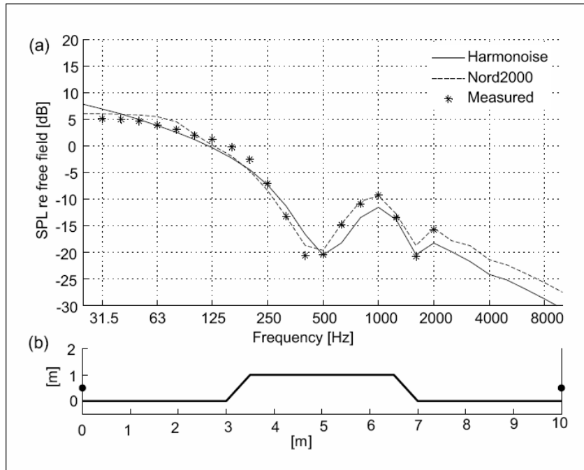
Figure 6. (a) Predicted results compared with reference data for test case 6: Sound propagation over 10 m of flat, acoustically soft ground with no refraction and no turbulence, and a 4 m wide, 1 m high hill with two diffracting edges and a 3 m wide acoustically hard top surface, blocking direct sound. Source height: 0.5 m; receiver height: 0.5 m; flow resistivity of the ground and sides of the hill: 200 kNs/m 4 . (b) Terrain profile.
