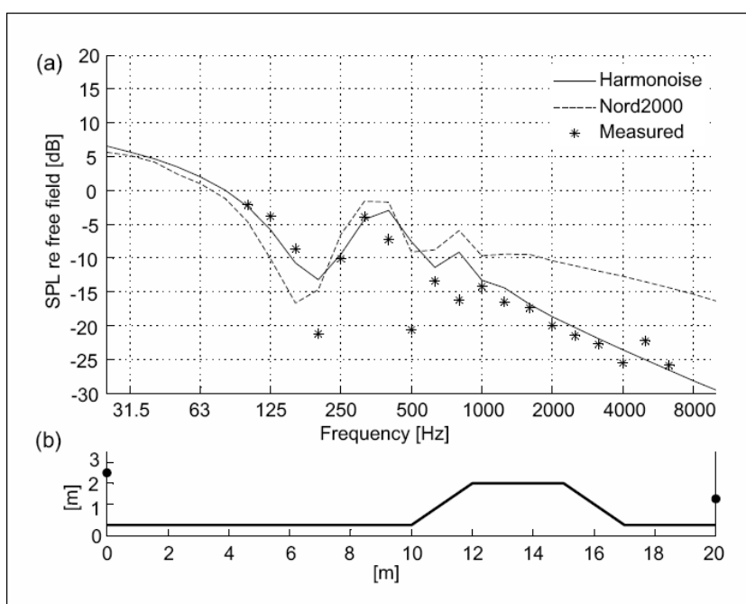
Figure 8. (a) Predicted results compared with reference data for test case 8: Sound propagation over 20 m of flat, acoustically hard ground with no refraction and no turbulence, and a 7 m wide, 2 m high hill with two diffracting edges and a 3 m wide acoustically soft top surface, blocking direct sound. Source height: 2.5 m; receiver height: 1.25 m; flow resistivity of top of hill: 63 kNs/m 4 . (b) Terrain profile.
