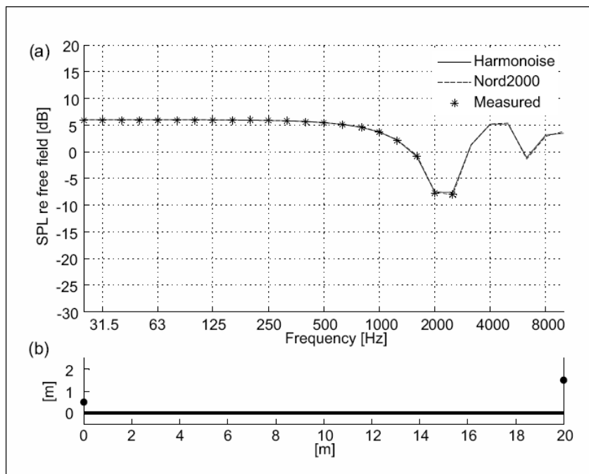
Figure 1. (a) Predicted results compared with reference data for test case 1: Sound propagation over 20 m of flat, acoustically hard ground with no refraction and no turbulence. Source height: 0.5 m; receiver height: 1.5 m. (b) Terrain profile.
