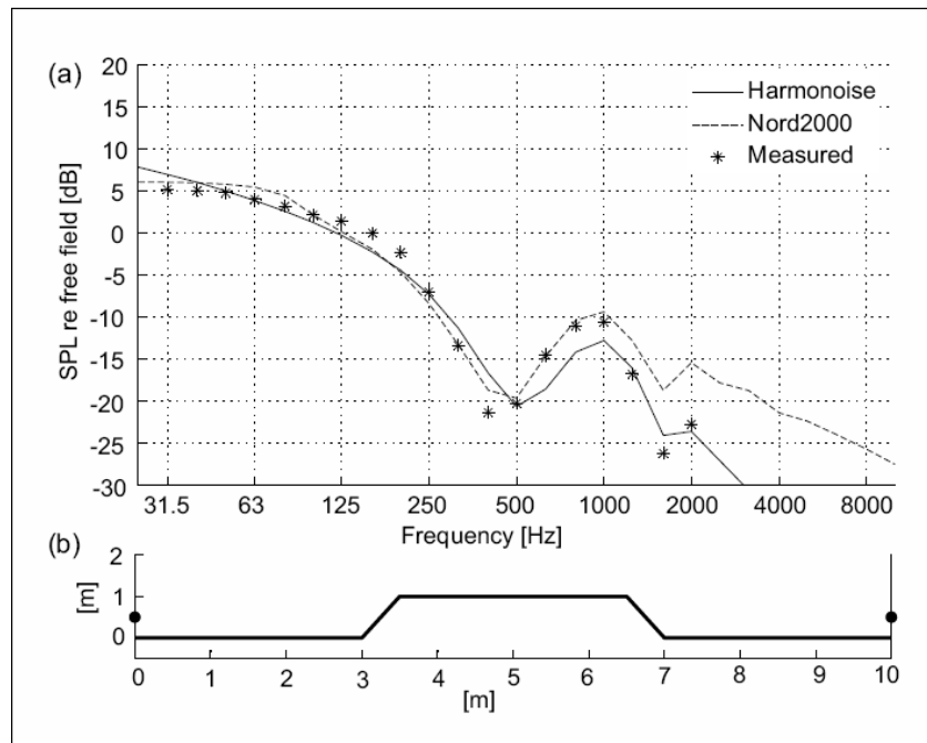
Figure 7. (a) Predicted results compared with reference data for test case 7: Sound propagation over 10 m of flat, acoustically soft ground with no refraction and no turbulence, and a 4 m wide, 1 m high hill with two diffracting edges and a 3 m wide acoustically soft top surface, blocking direct sound. Source height: 0.5 m; receiver height: 0.5 m; flow resistivity of all surfaces: 200 kNs/m 4 . (b) Terrain profile.
