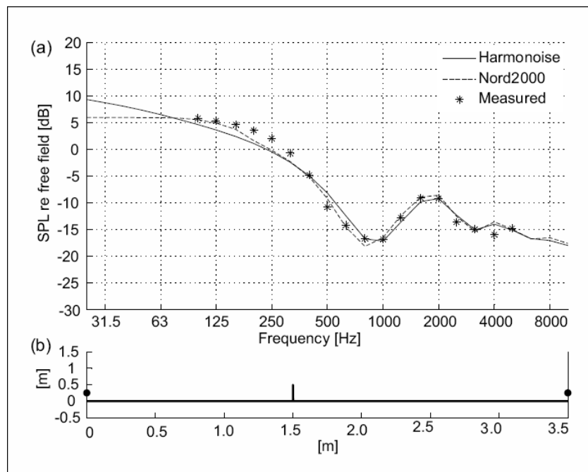
Figure 3. (a) Predicted results compared with reference data for test case 3: Sound propagation over 3.5 m of flat, acoustically soft ground with no refraction but some turbulence, and a thin, rigid barrier, blocking direct sound. Source height: 0.25 m; receiver height: 0.25 m; barrier height: 0.5 m; flow resistivity of the ground: 200 kNs/m 4 ; wind turbulence strength: 0.12 m 4/3 /s 2 ; temperature turbulence strength: 0.008 K/s 2 . (b) Terrain profile.
