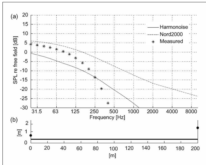
Figure 5. (a) Predicted results compared with reference data for test case 5: Sound propagation over 200 m of flat, acoustically hard ground with upward refraction caused by wind and no turbulence. Source height: 0.5 m; receiver height: 1.5 m; wind speed: -4.615 m/s. (b) Terrain profile.
