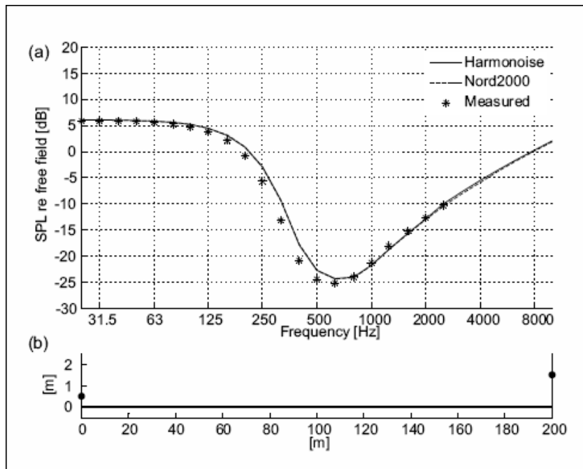
Figure 2. (a) Predicted results compared with reference data for test case 2: Sound propagation over 200 m of flat, acoustically soft ground with no refraction and no turbulence. Source height: 0.5 m; receiver height: 1.5 m; flow resistivity: 250 kNs/m 4 . (b) Terrain profile.
