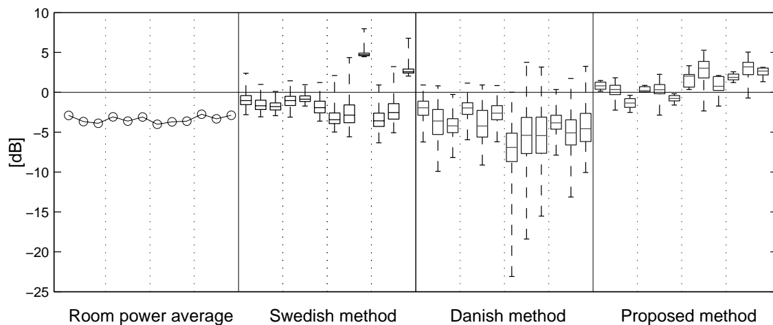
Figure 4: Summary of results given relative to the L10 target for each room and signal: Room power average, SE method (range, quartiles, median), DK method (range, quartiles, median) and the proposed method (range, quartiles, median). For each method, results are ordered by signal (31.5/33 Hz tone, 31.5 Hz third-octave noise, 125 Hz tone, 125 Hz third-octave noise – separated by dashed lines) and for each signal by room (office, living room, bedroom).
