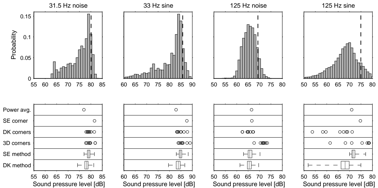
Figure 3: Measurements in office. Upper frames: Histograms of scannings (dashed line indicates L10, see Discussion); Lower frames: Room power average levels, levels of SE, DK and 3D corners, results of SE method and DK method
