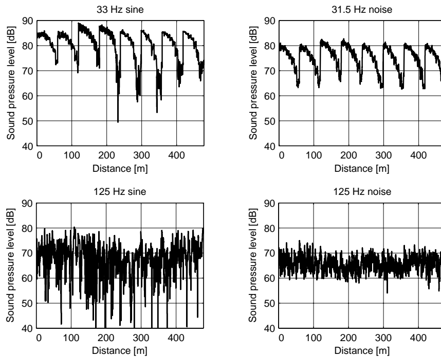
Figure 2: Scanning measurement in the office. Top: 33 Hz sinusoidal signal (left), 31.5 Hz third octave band filtered pink noise signal (right). Bottom: 125 Hz sinusoidal signal (left) and 125 Hz third octave band filtered pink noise (right).
